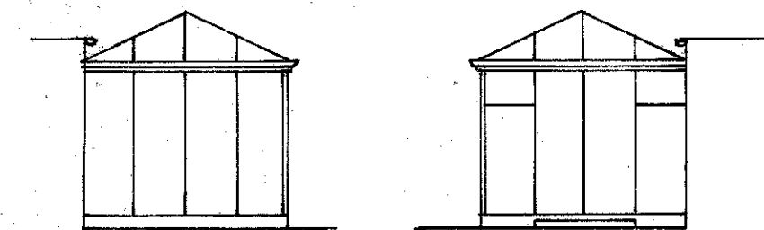
EXISTING CONSERVATORY SIDES 1:100
