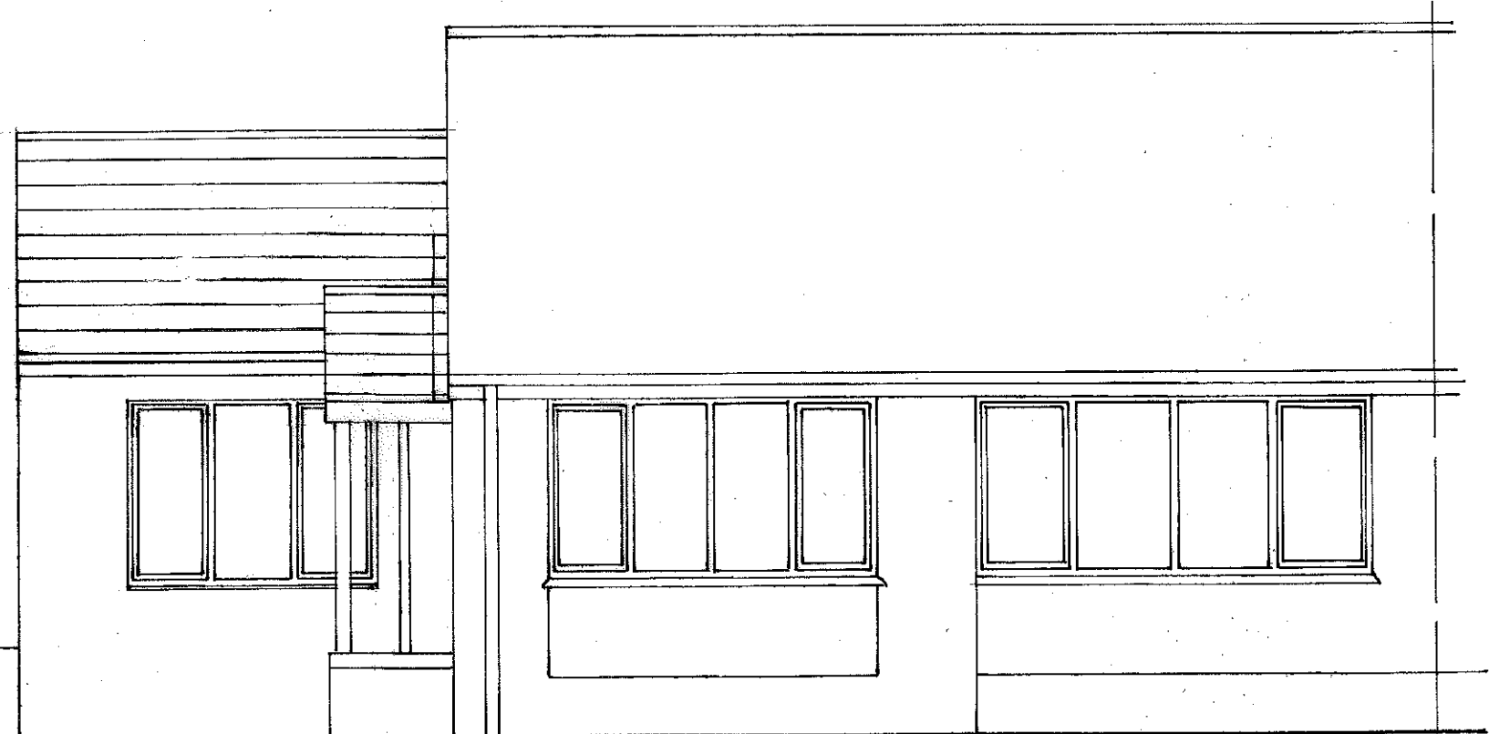
PROPOSED FRONTAGE 1:50
